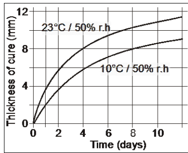
Diagram 1: Curing speed for Sikaflex®-211
